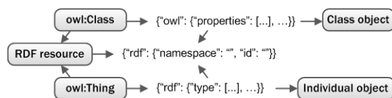
Figure 1: Mapping OWL to JSON.
